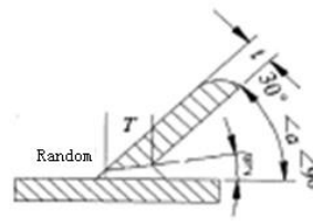
Section C
