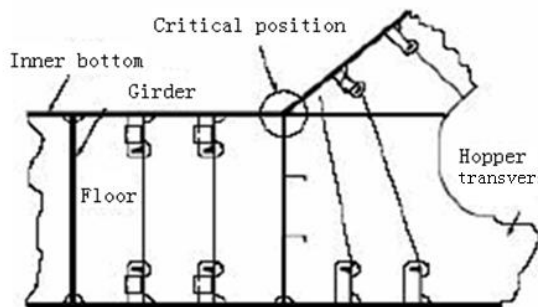
(1) Connection of sloped inner bottom/inner bottom/hopper tank girder
