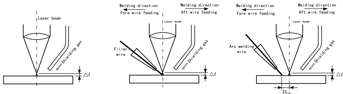
(1) Laser beam welding (Self-fusion welding) (2) Laser beam welding (Filler wire welding) (3) Laser-arc hybrid welding
