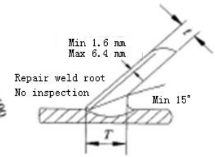
Section C'
