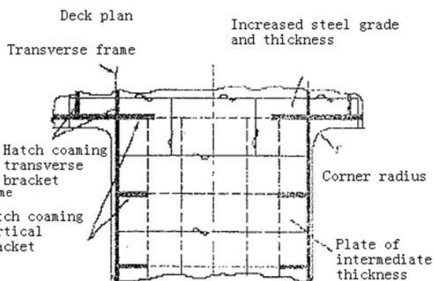
(2) Transition between different plate thicknesses of hatch corners and both sides
