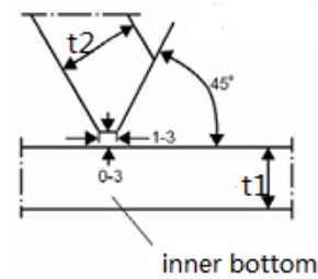
Figure 6A.1 Joint design between lower sloping plate, bulkhead stool sloping plate and inner bottom
