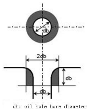
Figure 7A.4.3(1) Zones for magnetic particle/liquid penetrant testing on crankshafts
