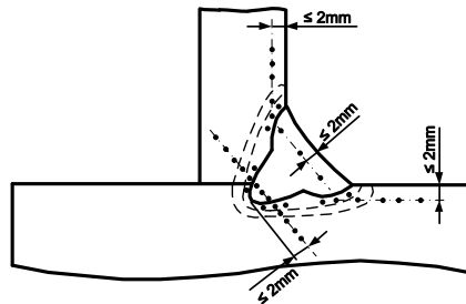
Figure 4.6.4.5 Example of arrangement of hardness test points for incomplete penetration fillet weld
