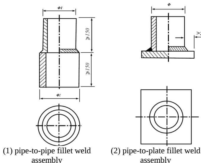
Figure 4.3.3.1 Fillet weld assembly of copper alloy pipe
