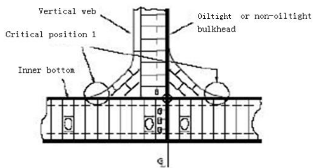
(4) Connection of end bracket toe end of centerline bulkhead vertical web to double bottom floor
