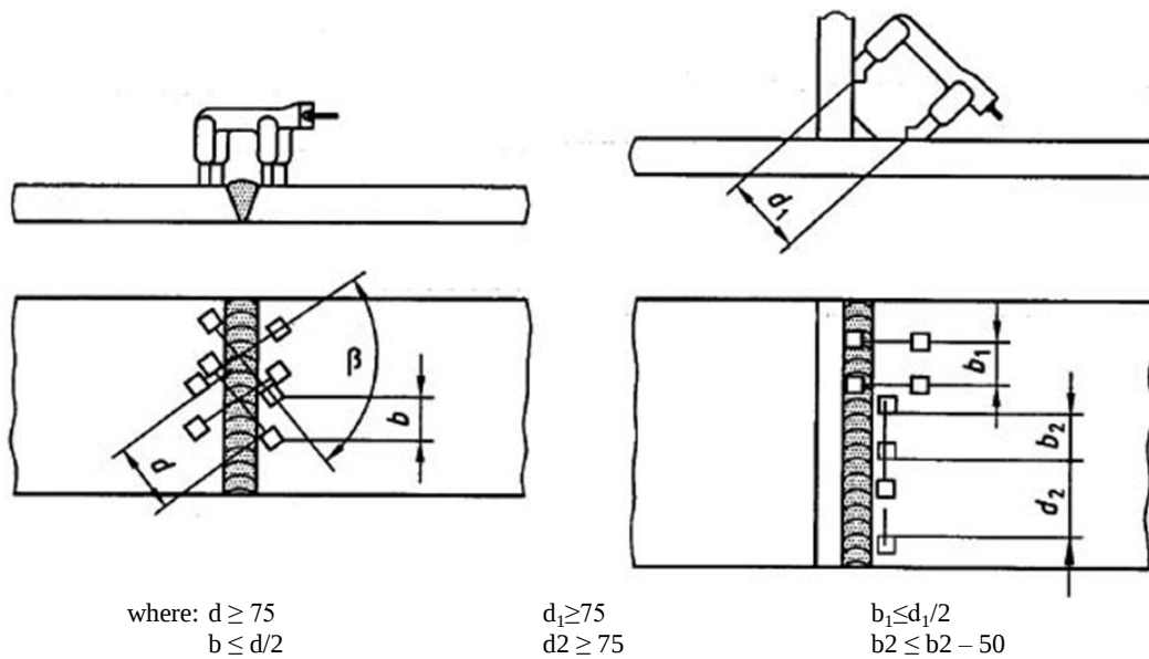
a. Magnetic particle testing of butt weld
