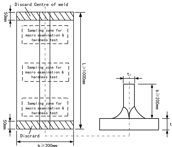
Figure 4.6.2.1 Diagram of full penetration fillet weld test assembly and sampling positions
